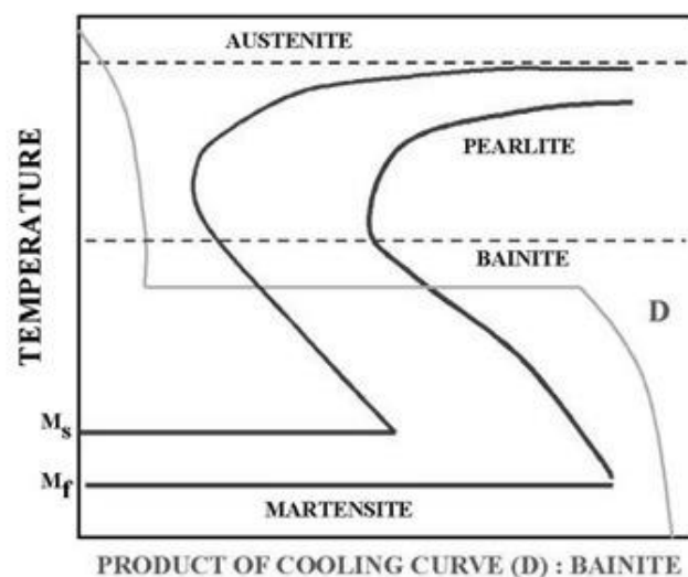
Figure 2.10 Interrupted Quench
