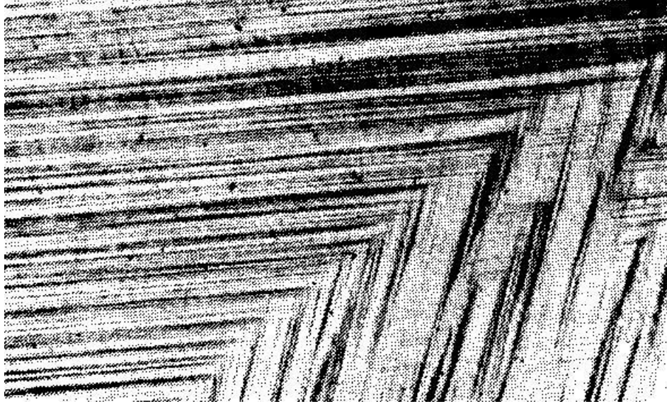
Figure 5.3 Slip lines in copper.
