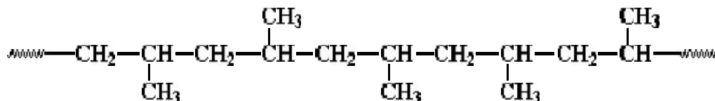
atactic polypropylene
