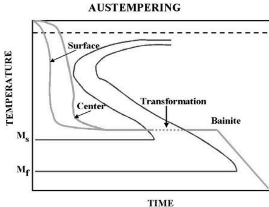
Figure 2.20 Austempering process.
