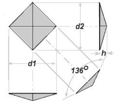
Vickers Pyramid Diamond Indenter Indentation
