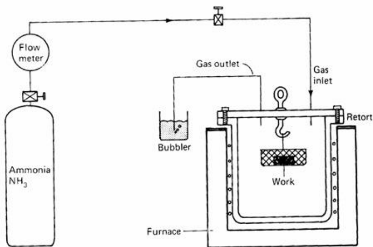
Figure 2.30 Nitriding process
